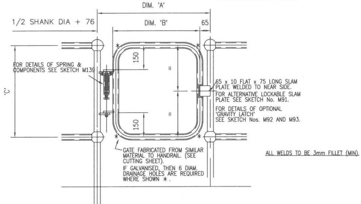
ELEVATION ON GATE (FROM PLATFORM SIDE).
